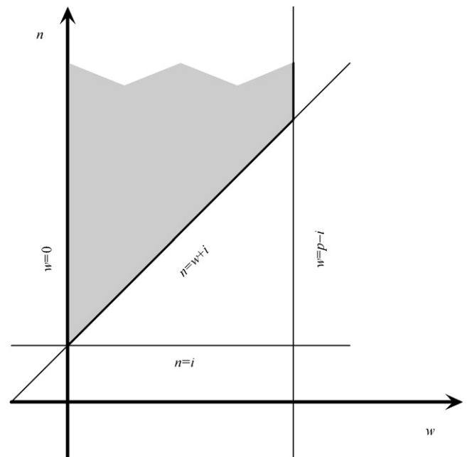
Fig. 7. The geometry of the summational transformation: \sum_{w=0}^{\min[(p-i),(n-i)]} \sum_{n=w+i}^{\infty} = \sum_{n=i}^{\infty} \sum_{w=0}^{\min[(p-i),(n-i)]} .
